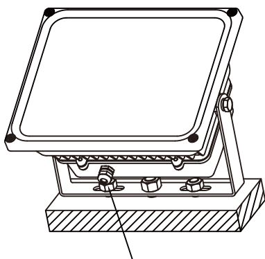
Fix the bracket on the installed surface.
