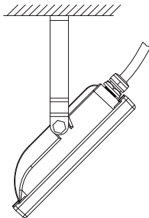
1.Ceiling installation
